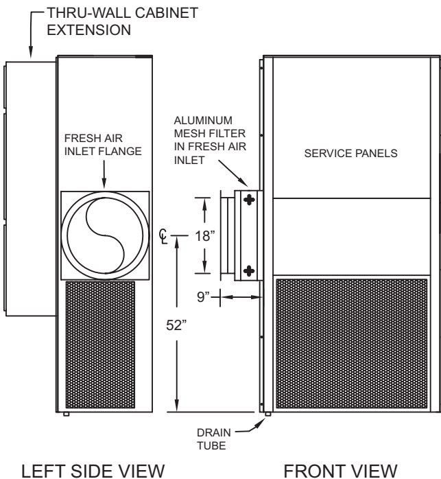
INLET FLANGE FOR HORIZONTAL FRESH AIR STACK CONNECTION
